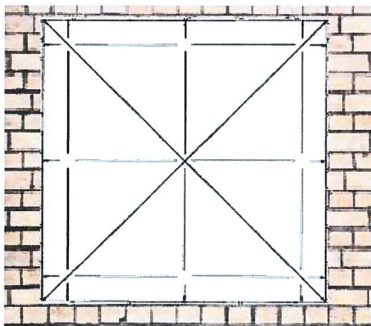
Figure 1 - Squareness measurements
